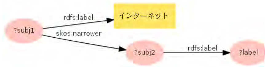
Figure 3: A partial graph pattern where the variables 'subj2' and 'label' represent the narrower term and its label.
